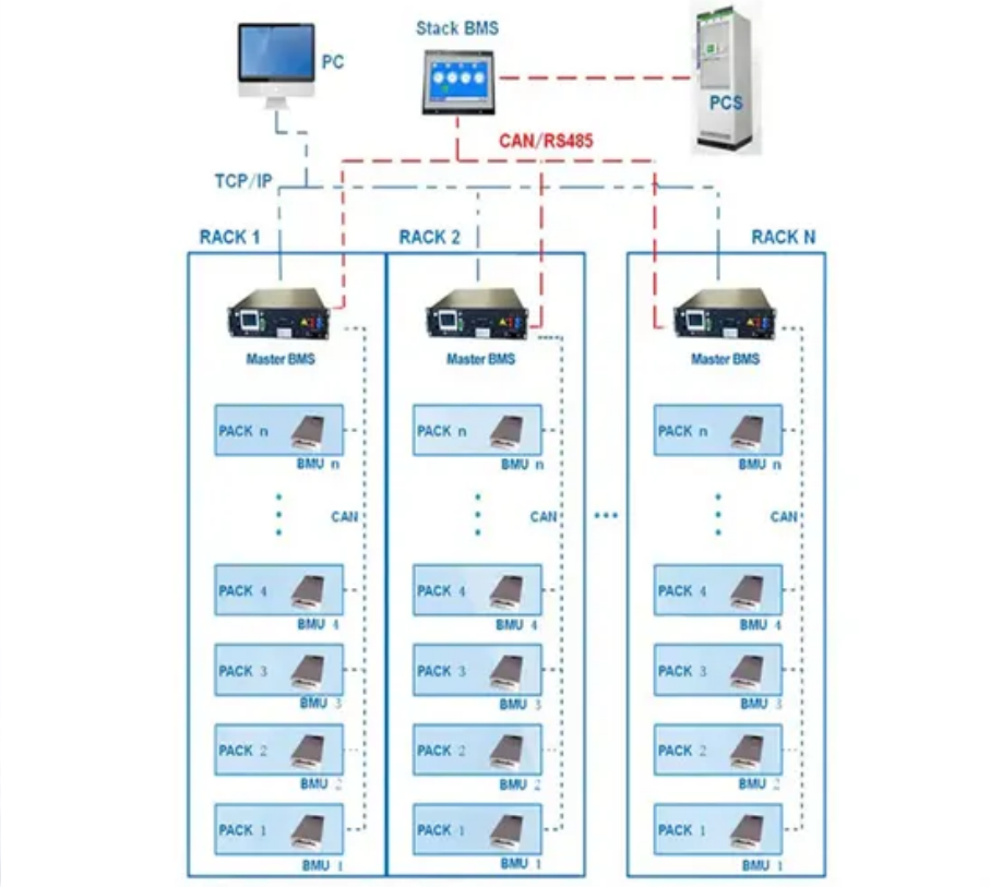
BMS Wiring Diagram
